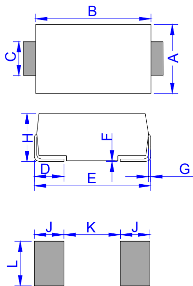
DO-214AA (SMB)
